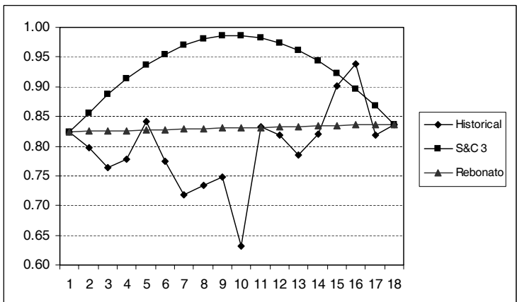
Fig. 6.7. Corresponding sub-diagonals
